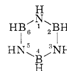
borazine
