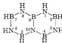
borazanaphthalene
