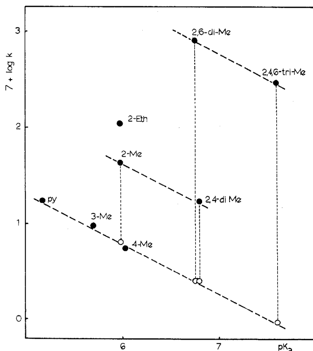
Figure 1.—Correlation between solvolysis rate and base strength (30°): ●, experimental points; O, expected in the absence of strain.
