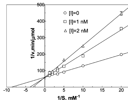
Figure 2. Reciprocal plot of the initial rate of the hGlxI reaction versus concentration of GSH-methylglyoxal thiohemiacetal substrate (S) at different fixed concentrations of [CHG( \beta -ala) n ] 2 substrate diamide [I]. Conditions: 50 mM sodium phosphate buffer, pH 7.0, 25 °C.
