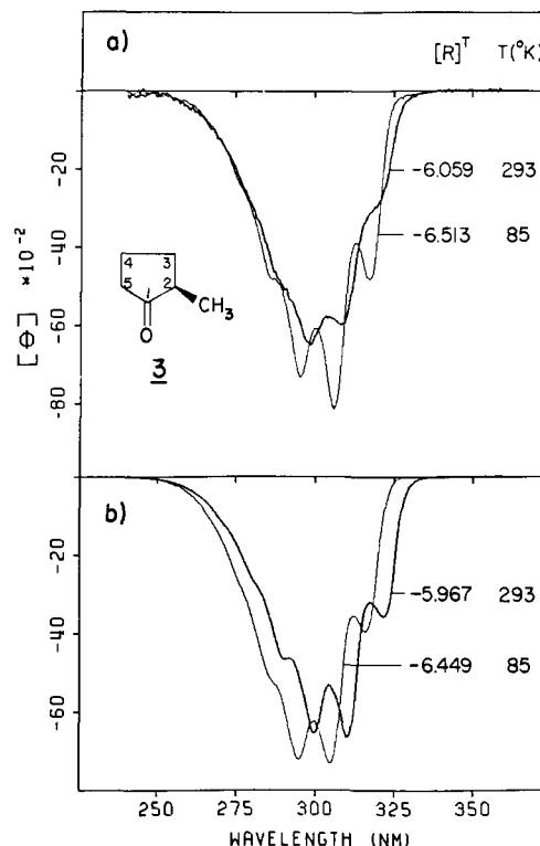
Figure 2. Circular dichroism spectra of (R)\text{-2-methylcyclopentanone (3)} (a) in EPA (ether-isopentane-ethanol 5:5:2) and (b) in IPM (isopentane-methylcyclohexane 4:1) at room temperature and 85 K.
