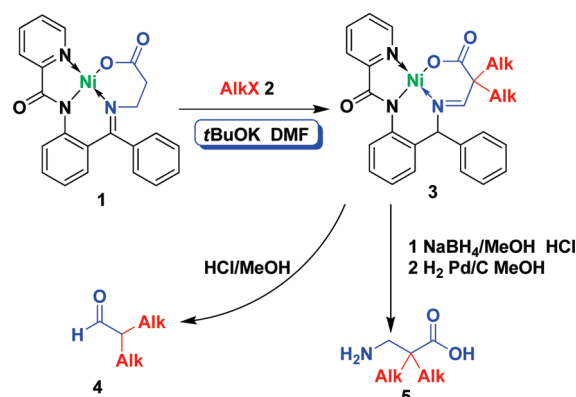
SCHEME 1. Synthesis of \alpha,\alpha -Disubstituted \beta -Amino Acids and \alpha,\alpha -Disubstituted Aldehydes via a Ni(II) Complex
