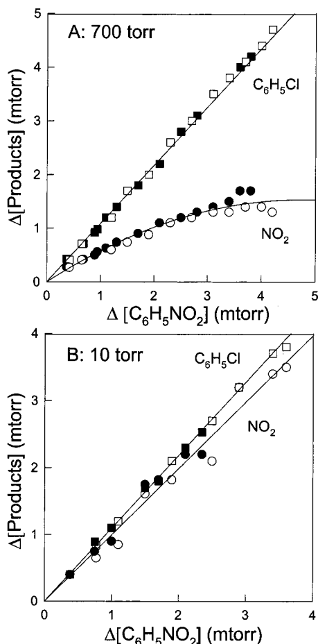
Figure 3. Yield of C 6 H 5 Cl (squares) and NO 2 (circles) versus loss of C 6 H 5 NO 2 in 700 (A) or 10 (B) Torr of either N 2 (open symbols) or air (filled symbols).
