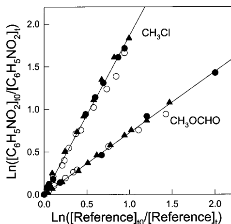
Figure 1. Decay of \text{C}_6\text{H}_5\text{NO}_2 versus the reference compounds ( \text{CH}_3\text{Cl} or \text{CH}_3\text{OCHO} ) in the presence of Cl atoms in 700 (circles) or 10 Torr (triangles) total pressure of either air (filled symbols) or \text{N}_2 (open symbols) diluent.
