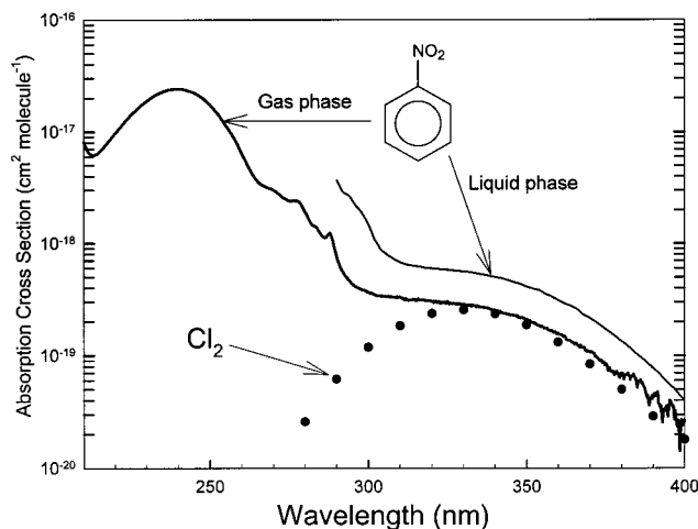
Figure 4. UV–visible spectrum (base e) of C 6 H 5 NO 2 in the gas phase (thick line, this work) and in liquid hexane (thin line). 1 The circles show the absorption spectrum of Cl 2 . 4
