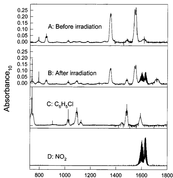
Figure 2. IR spectra obtained before (A) and after (B) 80 s of irradiation of a mixture of 4.7 mTorr \text{C}_6\text{H}_5\text{NO}_2 and 100 mTorr \text{Cl}_2 in 700 Torr of air. Panels C and D are reference spectra of \text{C}_6\text{H}_5\text{Cl} and \text{NO}_2 , respectively.
