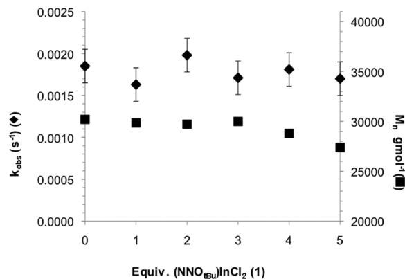
Figure 9. Plots of k_{\text{obs}} ( \blacklozenge ) observed PLA M_n ( \blacksquare ) as functions of added 1 for polymerization of LA with catalysts 5 ( [\text{5}] = 0.0024 \text{ M} , \text{CD}_2\text{Cl}_2 , room temperature; M_n = number averaged molecular weight).
