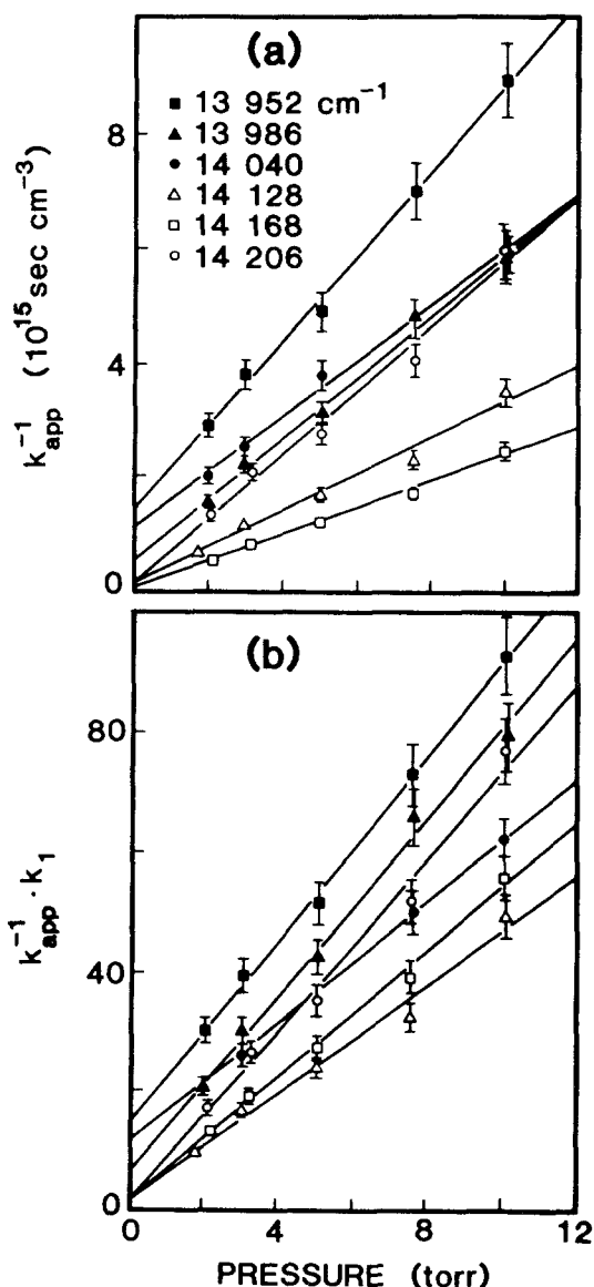
FIG. 5. Photolysis data in the 5–0 C–H stretch region: (a) Stern–Volmer plot; (b) reduced Stern–Volmer plot. Data are shown with 7% error bars.
