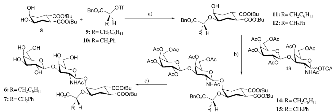
Scheme 3. Synthesis of 6 and 7 . a) \text{Bu}_2\text{SnO} , benzene, reflux; then \text{CsF} , DME, and 9 or 10 ; b) 13 (0.5 equiv) and \text{TfOH} (0.05 equiv) in \text{CH}_2\text{Cl}_2 , RT \rightarrow reflux; c) \text{H}_2/\text{Pd-C} , \text{MeOH} ; then cat. \text{MeONa} in \text{MeOH} . Bn = benzyl, DME = 1,2-dimethoxyethane, TCA = trichloroacetic acid, Tf = triflate = trifluoromethanesulfonyl.
