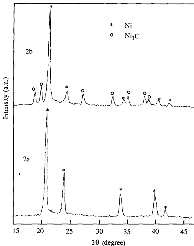
Fig. 2. XRD ( \text{MoK}\alpha ) profiles of Ni powder (a) (2a) and Ni powder (b) (2b).
