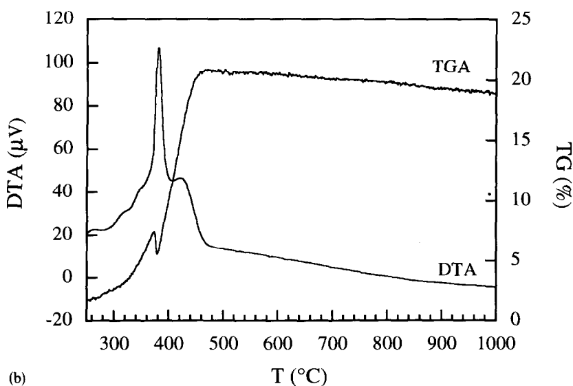
Fig. 1. TGA-DTA patterns of Ni powder (a) (1a) and Ni powder (b) (1b).
