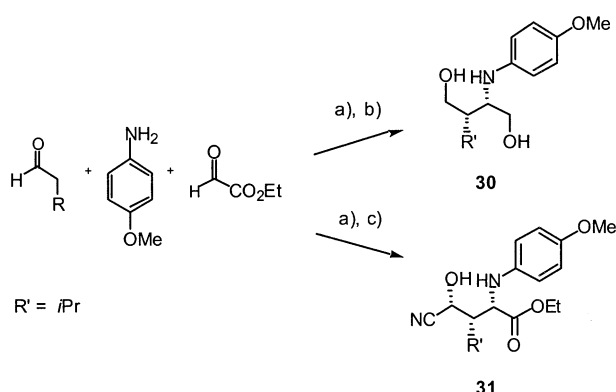
Scheme 4. One-pot direct catalytic asymmetric synthesis of functional \alpha -amino acid derivatives. i: a) Ethyl glyoxylate, 2 equiv isovaleraldehyde, 1.1 equiv p -anisidine, 10 mol % ( S )-proline, 4 °C. ii: either b) LAH, THF, 0 °C, 85 % yield two steps, or c) Et 2 AlCN, THF, –75 °C, 66 % yield two steps.
