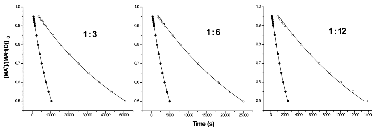
Fig. 5 Fit of experimental extent of reaction–time profiles to theoretical data for the reactions of MAH(D) (0.0015 M) with BQCN + at different concentrations in acetonitrile at 299 K. Experimental data for MAH are shown as solid and that for MAD as open circles with theoretical data represented by the solid lines. Ratios of initial reactant concentrations ([BQCN + ] 0 /[MAH(D)] 0 ) are specified on the plots.
