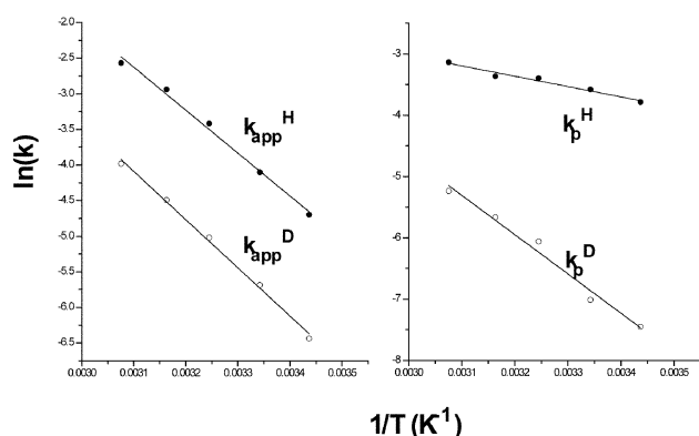
Fig. 4 Arrhenius plots for the reactions of MAH(D) (0.0015 M) with BQCN + (0.009 M) derived from k_{\text{app}}^{\text{H(D)}}(\text{M}^{-1} \text{s}^{-1}) and k_{\text{p}}^{\text{H(D)}}(\text{s}^{-1}) .
