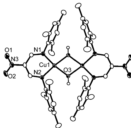
Figure 9. X-ray crystal structure representation of [\text{NO}_2(\text{H}_2\text{L}^{\text{Me2Me}})\text{Cu}]_2\text{-(}\mu\text{-OH)}_2 . All atoms are shown as 50% thermal ellipsoids with only heteroatoms labeled and hydrogen atoms and solvent molecules omitted for clarity (except for the hydrogen atoms on the hydroxo bridge).
