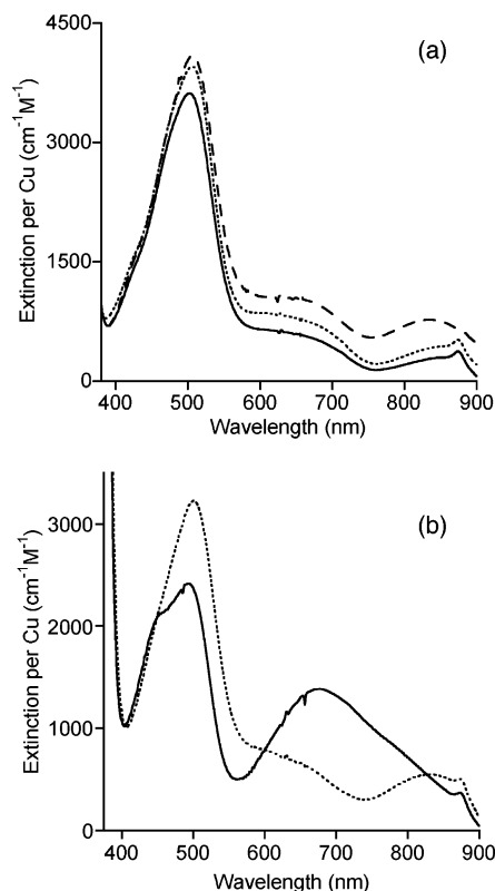
Figure 6. (a) UV-vis spectra of [H(Me_2L^{Et_2})CuCl]_n in toluene at 22.4 °C (—) and -49.8 °C (····), overlaid with the spectrum of H(Me_2L^{iPr_2})CuCl in CH_2Cl_2 (- - -). 7a (b) UV-vis spectra of [Cl(Me_2L^{Me_2})CuCl]_2 in toluene at 22.4 °C (····) and -55.0 °C (—).
