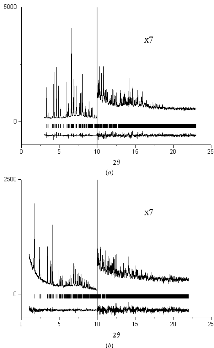
Figure 3 Rietveld plots for \text{LiNCS}\cdot\text{HL} (top) and \text{CuL}_2 (bottom).
