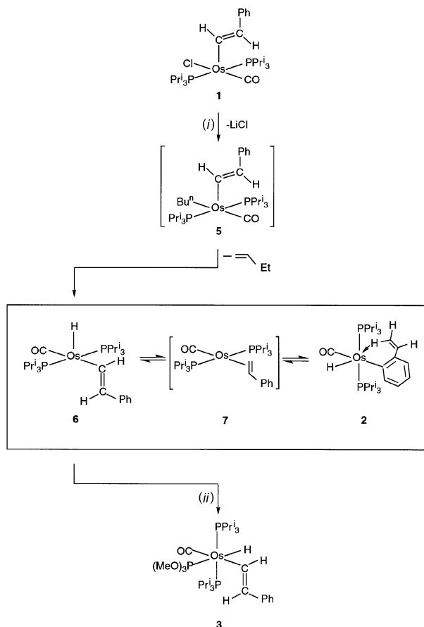
Scheme 4 (i) \text{LiBu}^n ; (ii) \text{P(OMe)}_3
