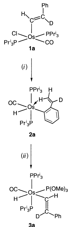
Scheme 5 (i) \text{LiBu}^n ; (ii) \text{P(OMe)}_3
