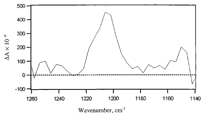
Figure 1. TRIR spectrum produced upon LFP (355 nm) of 2 from 0 to 200 ns in heptane at ambient temperature.
