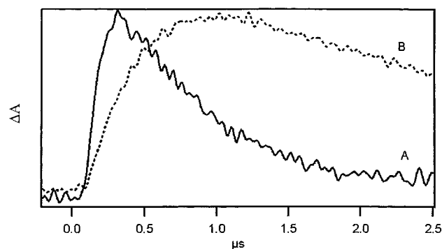
Figure 3. Decay of transient absorption at 1206 cm -1 (A) and the growth of transient absorption at 1316 cm -1 (B) following LFP (355 nm) of 2 in CCl 4 .
