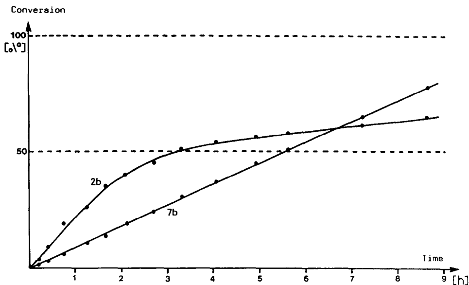
FIGURE 1: Enzymatic hydrolysis of 2b and 7b using Candida cylindracea lipase.
