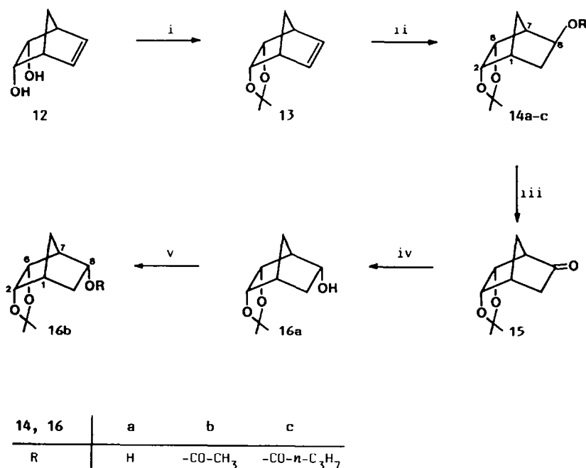
SCHEME III: Synthesis of compounds of type E and F.
