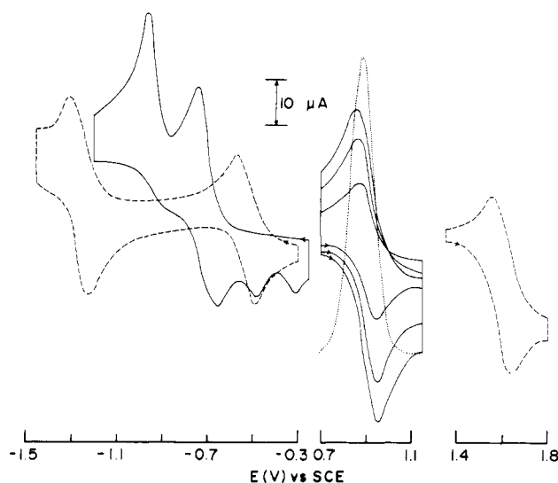
Figure 2. Segmented voltammograms in acetonitrile (0.1 M TEAP) at platinum electrode (298 K). Region 1.8–1.4 V: ---, dc cyclic of [Ru(bpy) 2 ](tap)](ClO 4 ) 2 ·H 2 O at a scan rate of 50 mV s -1 . Region 1.1–0.7 V: —, dc cyclic of RuCl 2 (tap) 2 at three different scan rates (100, 300, and 500 mV s -1 ); ---, phase-sensitive ac cyclic of RuCl 2 (tap) 2 at a sinusoidal frequency of 22 Hz and a dc scan rate of 0.5 mV s -1 . Region -0.3 to -1.5 V: —, dc cyclic of RuCl 2 (tap) 2 at a scan rate of 50 mV s -1 ; ---, dc cyclic of [Ru(bpy) 2 ](tap)](ClO 4 ) 2 ·H 2 O at a scan rate of 50 mV s -1 .
