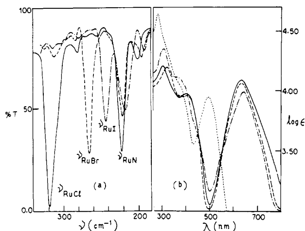
Figure 1. (a) Far-IR spectra of \text{RuX}_2(\text{pap})_2 in polyethylene disk: —, \text{X} = \text{Cl} ; ---, \text{X} = \text{Br} ; - · -, \text{X} = \text{I} . (b) Visible-UV spectra of \text{RuX}_2(\text{pap})_2 in dichloromethane: —, \text{X} = \text{Cl} ; ---, \text{X} = \text{Br} ; - · -, \text{X} = \text{I} . Visible-UV spectra of [\text{Ru}(\text{bpy})_2(\text{pap})](\text{ClO}_4)_2 \cdot \text{H}_2\text{O} in acetonitrile: ....
