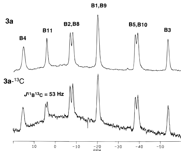
Figure 11. The ^{11}\text{B}\{^1\text{H}\} NMR spectra of hypho -12- \text{CH}_3 -12,13- ^{13}\text{CNB}_9\text{H}_{15} ( 3a- ^{13}\text{C} ) and hypho -12- \text{CH}_3 -12,13- \text{CNB}_9\text{H}_{15} ( 3a ).
