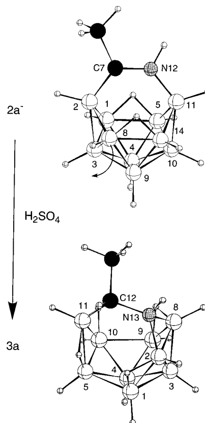
Figure 8. Comparison of the structures of 2a^- and 3a .
