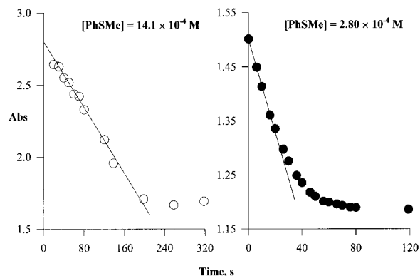
Figure 1. Variation of absorbance at 270 nm with time for reaction of thioanisole at 25.0°C, 0.1 M H 2 O 2 , 0.001 M NaOH in H 2 O–MeCN (95:5, v/v) for 14.1 \times 10^{-4} (○) and 2.80 \times 10^{-4} (●) M PhSMe
