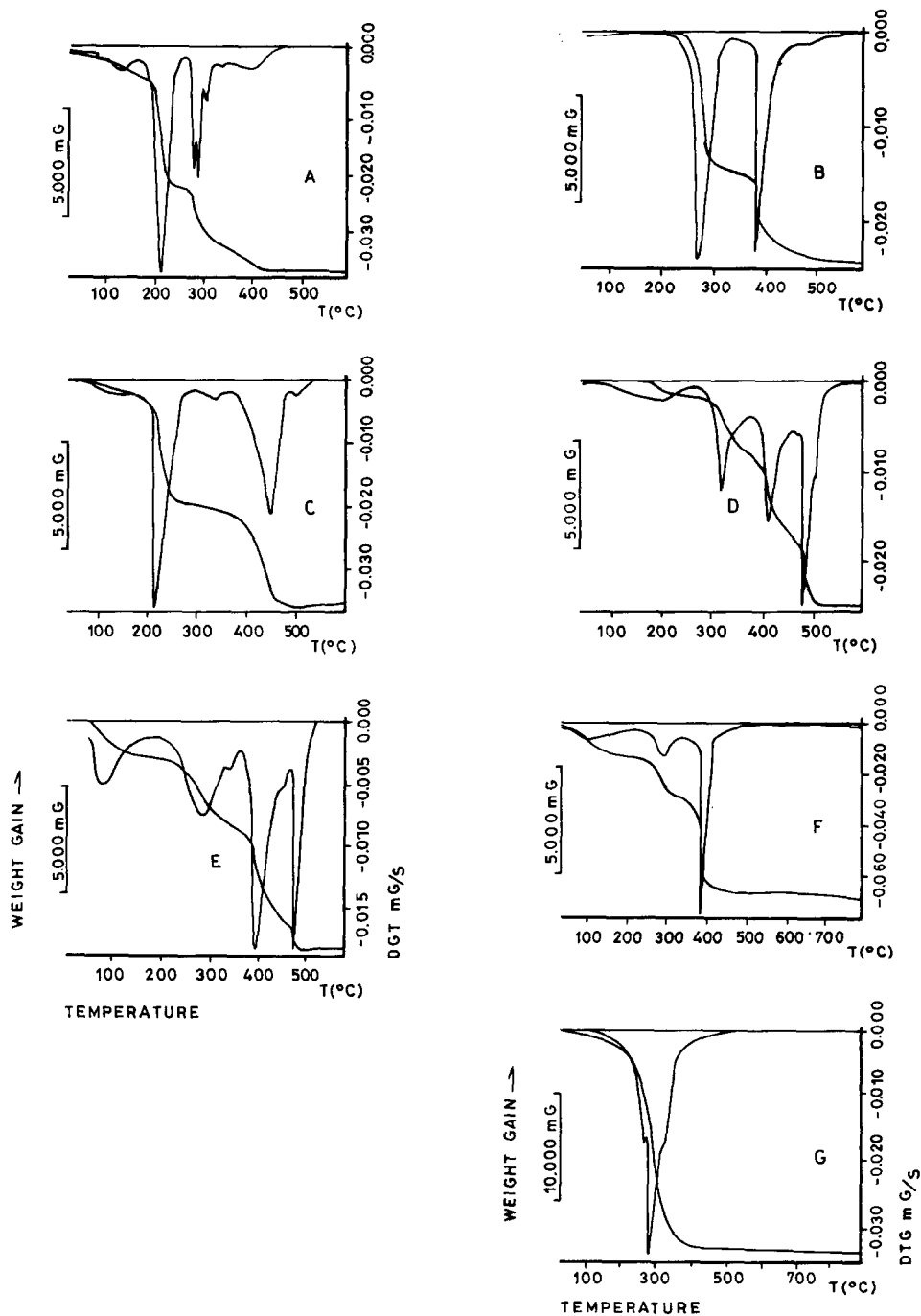
Fig. 1. TG curves of 5,5'-methylenebisthiosalicylic acid complexes of: (A) Cu(II), (B) Pb(II), (C) Cd(II), (D) Mn(II), (E) Co(II), (F) Ni(II); and (G) 5,5'-methylenebisthiosalicylic acid.
