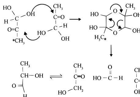
Scheme 8. Disproportionation of \alpha -Hydroxy Carbonyls and \alpha -Dicarbonyl Compounds a
