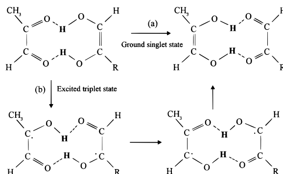
Scheme 8. Disproportionation of \alpha -Hydroxy Carbonyls and \alpha -Dicarbonyl Compounds a
