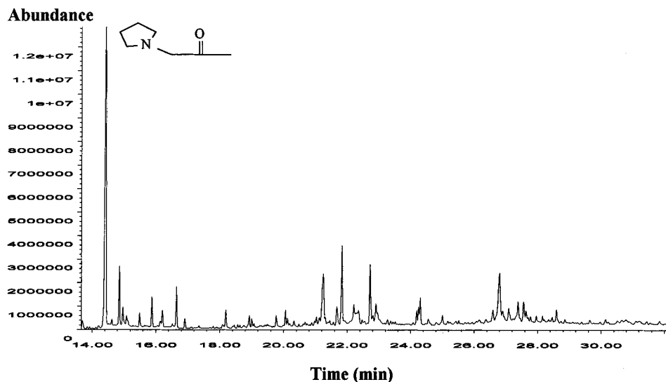
Figure 1. Pyrogram of 1-(proline)-1-deoxy-D-glyceraldehyde (7).
