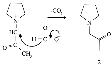
Scheme 6. Reduction Mechanism of Iminium Ions and Carbonyl Compounds by Formic Acid
