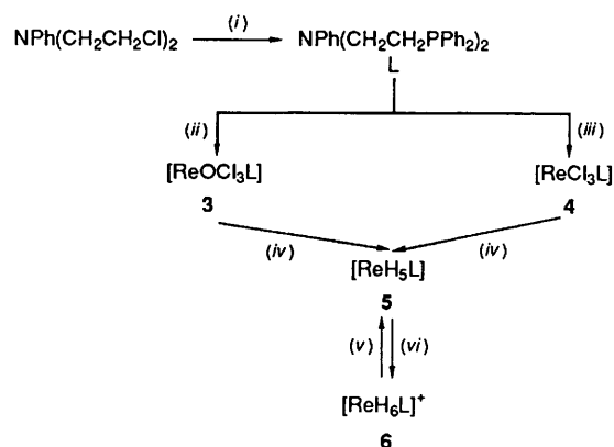
Scheme 1 (i) \text{LiPPh}_2 ; (ii) [\text{ReOCl}_3(\text{AsPh}_3)_2] ; (iii) [\text{ReCl}_3(\text{MeCN})(\text{PPh}_3)_2] ; (iv) \text{LiAlH}_4 ; (v) \text{H}^+ ; (vi) \text{NEt}_3 .
