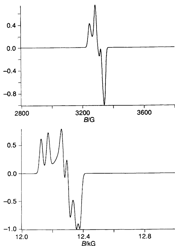
Fig. 8 Simulations of X- (top) and Q-band (bottom) ESR spectra (77 K) of oxidation products of [\text{Ag}([15]\text{aneS}_5)]^+
