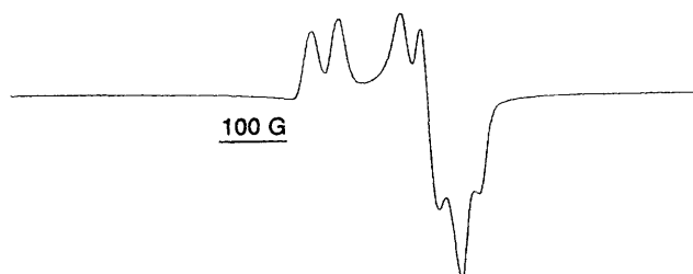
Fig. 7 Q-Band ESR spectrum (77 K) of the oxidation product of [\text{Ag}([15]\text{aneS}_5)]^+ in \text{H}_2\text{SO}_4 glass
