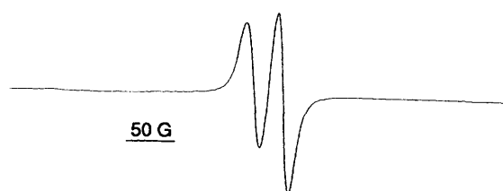
Fig. 6 X-Band ESR spectrum (298 K) of the oxidation product of [\text{Ag}([15]\text{aneS}_5)]^+ in \text{H}_2\text{SO}_4 solution
