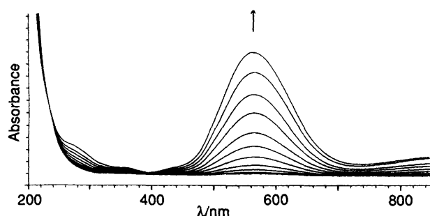
Fig. 4 In situ electronic spectrum for conversion of [\text{Ag}([15]\text{aneS}_5)]^+ into [\text{Ag}([15]\text{aneS}_5)]^{2+} (OTE, 243 K, +1.5 V vs. \text{Ag}-\text{Ag}^+ )
