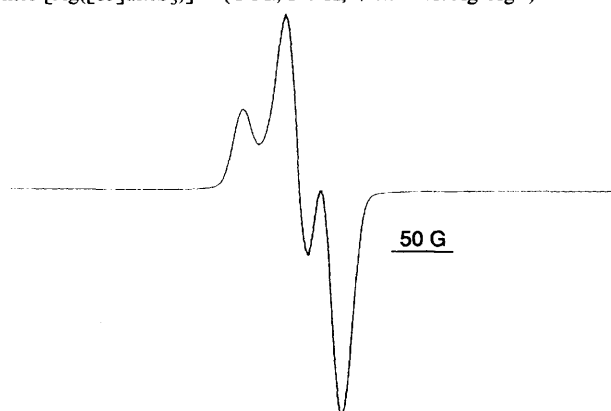
Fig. 5 X-Band ESR spectrum (77 K) of the oxidation product of [\text{Ag}([15]\text{aneS}_5)]^+ in \text{H}_2\text{SO}_4 glass
