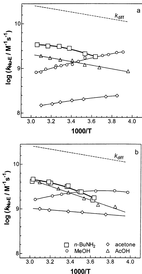
Figure 4. Arrhenius plots for reaction of 1a (a) and 1b (b) with n -BuNH 2 ( \square ), MeOH ( \circ ), acetone ( \diamond ), and AcOH ( \triangle ) in acetonitrile solution. Data for MeOH and AcOH: Reprinted from ref 18. Copyright 1997 National Research Council of Canada. Data for acetone: Reprinted from ref 21. Copyright 1998 American Chemical Society.
