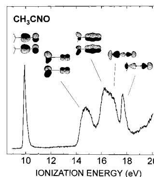
Figure 4. HeI photoelectron spectrum of CH 3 CNO and schematics of the corresponding molecular orbitals.
