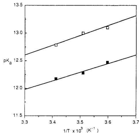
Figure 5. Temperature dependence of the pK a for the nicotinamide ribose diol (■) and the adenosine ribose diol (□) of NAD + as determined by 13 C NMR titration. Extrapolation of the pK a for the nicotinamide ribose diol up to 37 °C gives a pK a of 11.9 ± 0.1, consistent with the pK eq obtained at 37 °C from the pH-rate profile.
