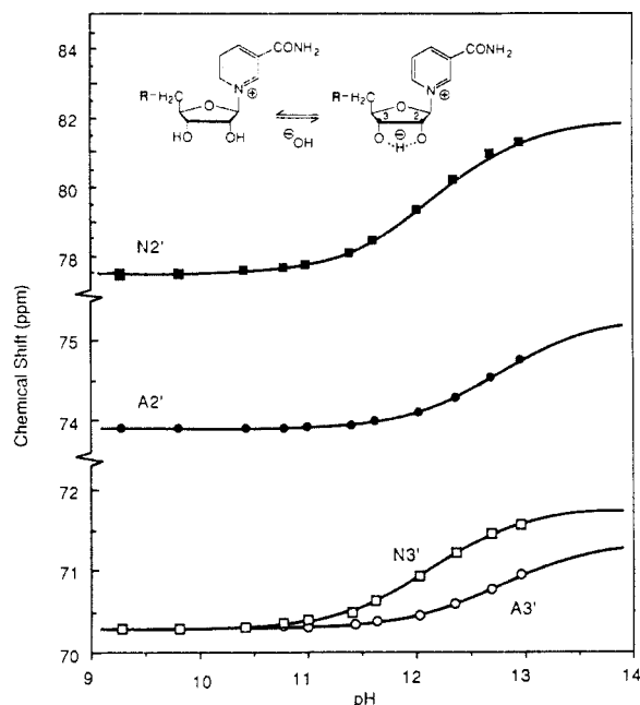
Figure 4. 13 C chemical shift vs pH for the nicotinamide ribose 2' (N2', ■) and 3' (N3', □) carbons and the adenine ribose 2' (A2', ●) and 3' (A3', ○) carbons of NAD + at 20 °C. Spectra were acquired as described in the text. Nonlinear least-squares analysis of the titration data yields a mean pK a of 12.15 ± 0.01 for the nicotinamide ribose diol and 12.77 ± 0.03 for the adenine ribose 2'- and 3'-carbons.
