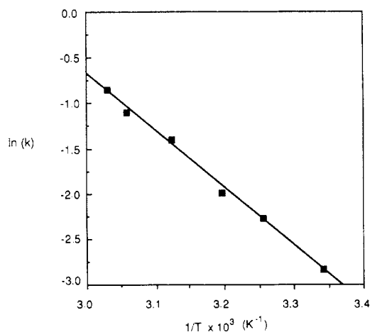
Figure 3. Temperature dependence of the rate of hydrolysis of the nicotinamide-glycosyl bond of NAD + at pH 13.4.
