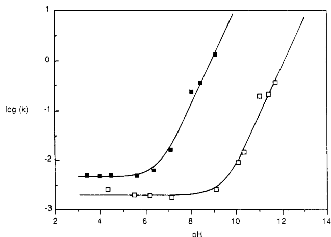
Figure 7. pH-rate profiles (low-pH region) for isopro-NR ^+ ( \square ) and \text{NAD}^+ ( \blacksquare ) at 80^\circ\text{C} . Below pH 7 the product of the reaction of isopro-NR ^+ is nicotinamide. Above pH 7 the product is 2-HPC. The product of \text{NAD}^+ hydrolysis is nicotinamide over the entire pH range.
