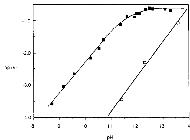
Figure 8. pH-rate profiles (high-pH region) for isopro-NR ^+ ( \square ) and \text{NAD}^+ ( \blacksquare ) at 37^\circ\text{C} . Data for the \text{NAD}^+ pH-rate profile are taken from Figure 1. The product of the reaction of isopro-NR ^+ is 2HPC, and the product of the reaction of \text{NAD}^+ is nicotinamide.
