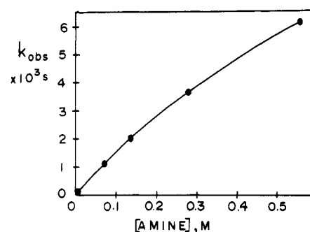
Figure 2. Plot of the observed pseudo-first-order rate constant for the reaction of the ( N -methyltetrakis( p -sulfophenyl)porphinato)-copper(II) anion with di- n -butylamine in acetonitrile at 44.5 °C vs. the concentration of di- n -butylamine.
