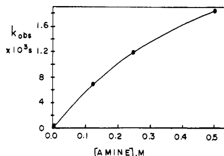
Figure 3. Plot of the observed pseudo-first-order rate constant for the reaction of ( N -methyldeuteroporphyrin IX dimethyl ester)-copper(II) with di- n -butylamine in acetonitrile at 44.2 °C vs. the concentration of di- n -butylamine.
