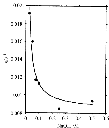
Fig. 3 Observed rate constants for the subsequent reaction of nitrile ylide 3b versus sodium hydroxide concentrations, in 60 : 40 water–dioxane; all substrate concentrations were 1.25 \mu\text{M} .
