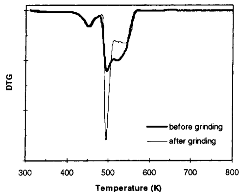
Fig. 8. Comparison between TPR profiles (DTG) of NiO 623 before and after grinding ( \beta = 0.033 \text{ K s}^{-1} ).
