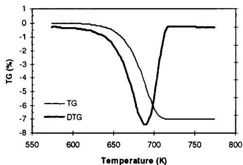
Fig. 1. TPR profiles (TG and DTG) of \text{Mn}_3\text{O}_4 1273 ( \beta = 0.033 \text{ K s}^{-1} ).
