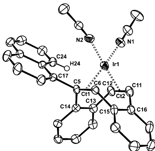
Figure 3. Structure of the cation [\text{Ir}(\text{Naphdbcot})(\text{MeCN})_2]^+ in 8b . Only the R -configured isomer is shown. Thermal ellipsoids are drawn at the 50% probability level; hydrogen atoms, the \text{SbF}_6^- anion, and a MeCN solvent molecule are omitted for clarity. Selected bond lengths (Å) and angles (deg): Ir1–C5 = 2.131(6), Ir1–C6 = 2.102(7), Ir1–ct1 = 1.990(7), Ir1–C11 = 2.126(8), Ir1–C12 = 2.103(8), Ir1–ct2 = 1.993(8), Ir1–N1 = 2.030(6), Ir1–N2 = 2.041(6), C5–C6 = 1.443(9), C11–C12 = 1.41(1); N1–Ir1–N2 = 90.3(3), N2–Ir1–Ct1 = 90.2(3), Ct1–Ir1–Ct2 = 88.6(3), Ct2–Ir1–N1(3) = 91.3. ct = centroids of the coordinated C=C units; \varphi = 6.7^\circ is the intersection angle of the ct1–Ir1–ct2 plane with the N1–Ir1–N2 plane. Torsion angles (deg): C5–C6–C15–C16 = 71.1(9), C15–C16–C11–C12 = –69(1), C11–C12–C13–C14 = 74(1), C13–C14–C5–C6 = –68.8(9); average 70.8^\circ .
