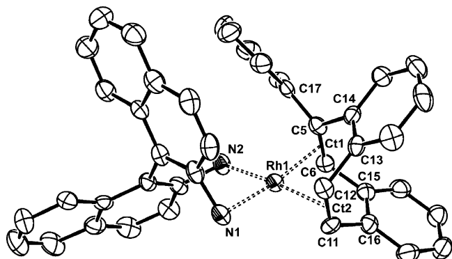
Figure 4. Structure of the cation [\text{Rh}((R)\text{-Phdbcot})((R)\text{-}(+)\text{-}1,1'\text{-binaphthyl-}2,2'\text{-diamine})]^+ in (R)\text{-}[(R)\text{-}(+)\text{-}]\textbf{11a} . Thermal ellipsoids are drawn at the 50% probability level; hydrogen atoms and the \text{CF}_3\text{SO}_3^- anion are omitted for clarity. Selected bond lengths (Å) and angles (deg): Rh1–C5 = 2.148(4), Rh1–C6 = 2.123(5), Rh1–ct1 = 2.016(5), Rh1–C11 = 2.121(4), Rh1–C12 = 2.121(5), Rh1–ct2 = 2.001(5), Rh1–N1 = 2.138(4), Rh1–N2 = 2.193(4), C5–C6 = 1.407(7), C11–C12 = 1.403(7); N1–Rh1–N2 = 87.7(1), N2–Rh1–Ct1 = 92.7(2), Ct1–Rh1–Ct2 = 88.0(2), Ct2–Rh1–N1 = 92.6(2) ct = centroids of the coordinated C=C units; \varphi = 11.5^\circ is the intersection angle of the ct1–Rh1–ct2 plane with the N1–Rh1–N2 plane. Torsion angles (deg): C5–C6–C15–C16 = 74.9(6), C15–C16–C11–C12 = –69.3(6), C11–C12–C13–C14 = 72.2(6), C13–C14–C5–C6 = –68.4(6); average 71.2^\circ .
