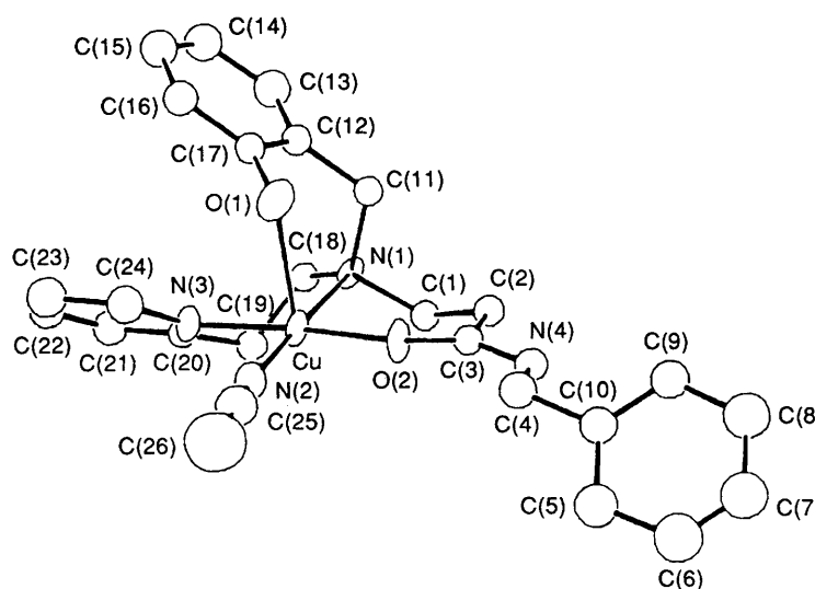
Fig. 4 An ORTEP perspective view of complex 4 (the triflate counter ions have been omitted for clarity)
