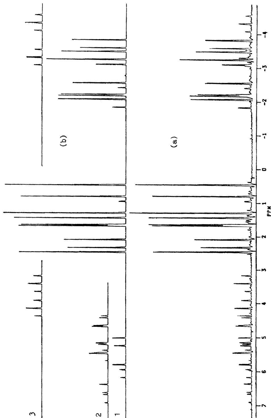
Fig. 1. Observed (a) and calculated (b) ^{31}\text{P}\{^1\text{H}\} spectrum of \text{RhC}(\text{PMe}_3)_3 ( \eta^2\text{-MVK} ): 1 \equiv I, 2 \equiv II, 3 \equiv [\text{Rh}(\text{PMe}_3)_4\text{O}_2]\text{Cl} .
