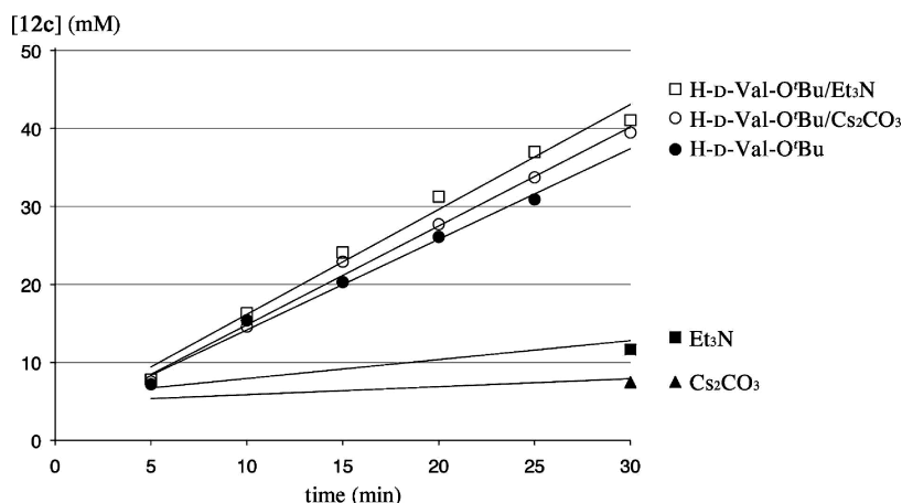
Figure 2. Kinetic profiles of the asymmetric amination of 7c promoted by \text{La}(\text{NO}_3)_3 \cdot 6\text{H}_2\text{O}/(R)\text{-3a}/\text{base} = 1/1/3 catalyst. The reactions were run with [\text{7c}] = 100 \text{ mM} , [\text{BocN}=\text{NBoc}] = 120 \text{ mM} , [\text{La}(\text{NO}_3)_3 \cdot 6\text{H}_2\text{O}] = 2.5 \text{ mM} , [(R)\text{-3a}] = 2.5 \text{ mM} , and [\text{base}] = 7.5 \text{ mM} (4 mol % of catalyst loading based on La ). \bullet : base = H-D-Val-O'Bu (corresponds to Table 4, entry 1), \blacksquare : base = \text{Et}_3\text{N} (entry 2), \blacktriangle : base = \text{Cs}_2\text{CO}_3 (entry 3), \square : base = H-D-Val-O'Bu/ \text{Et}_3\text{N} (1/2) (entry 4), \circ : base = H-D-Val-O'Bu/ \text{Cs}_2\text{CO}_3 (1/2) (entry 5).
