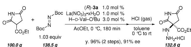
Scheme 4. One-Hundred Gram Scale Demonstration of the Second-Generation Catalytic Asymmetric Amination
