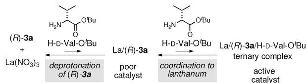
Scheme 8. Proposed Dual Role of Additional Amine Base in the Second-Generation Amination Reaction
