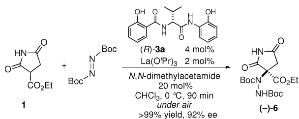
Scheme 3. First-Generation Amination Catalyst
