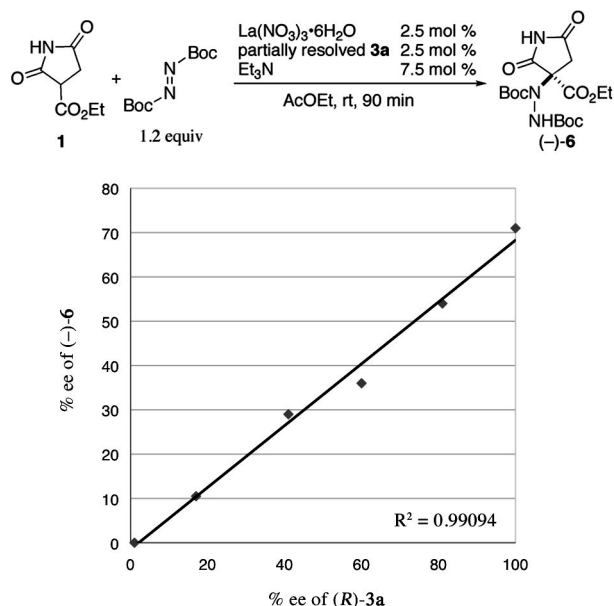
Figure 3. Plot of % ee of product (-)-6 versus % ee of ligand (R)-3a in the second-generation catalytic asymmetric amination using \text{Et}_3\text{N} as a base.
