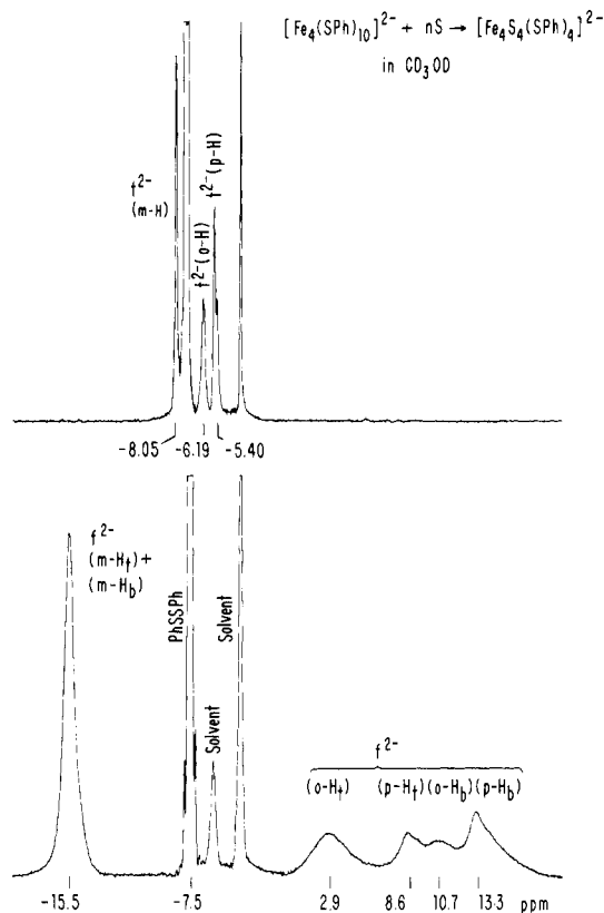
Figure 7. ^1\text{H} NMR spectra (100 MHz) of equilibrium solutions in \text{CD}_3\text{OD} at \sim 27^\circ\text{C} : bottom, \sim 0.05 M \text{Na}_2[\text{Fe}_4(\text{SPh})_{10}] ( f^{2-} , from \sim 0.20 M \text{FeCl}_3 + 3.5 equiv of \text{NaSPh} ); top, 1 h after addition of 4.0 equiv of sulfur/ f^{2-} , demonstrating formation of [\text{Fe}_4\text{S}_4(\text{SPh})_4]^{2-} ( t^{2-} ). Signal assignments are indicated.
