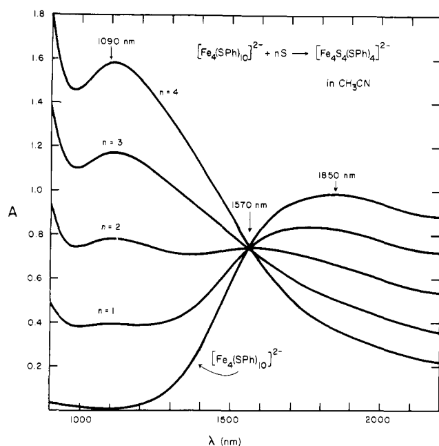
Figure 3. Near-infrared spectra of equilibrium solutions resulting from the reactions of 10.0 mM (Et 4 N) 2 [Fe 4 (SPh) 10 ] 2- with n = 1.0–4.0 equiv of sulfur at ~25 °C. Other details are as in Figure 2 except that spectra were measured 12–15 h after the addition of sulfur.
