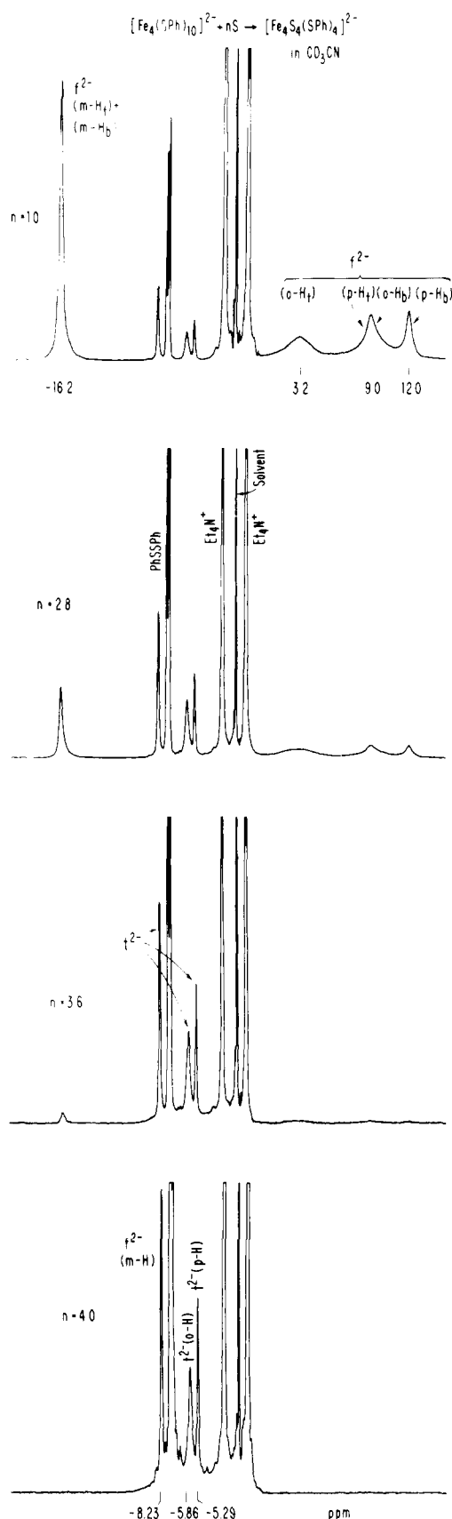
Figure 4. 1 H NMR spectra (100 MHz) of equilibrium solutions resulting from the reactions of (Et 4 N) 2 [Fe 4 (SPh) 10 ] 2- with 1.0–4.0 equiv of sulfur in CD 3 CN at ~27 °C, yielding [Fe 4 S 4 (SPh) 4 ] 2- (t 2- ). Each spectrum corresponds to a separate reaction system measured ~1 h after the addition of sulfur. Spectral amplitudes are not constant; signal assignments are indicated (cf. Figure 5). In this and other NMR spectra shifts (ppm) downfield and upfield of Me 4 Si reference are designated as - and +, respectively.
