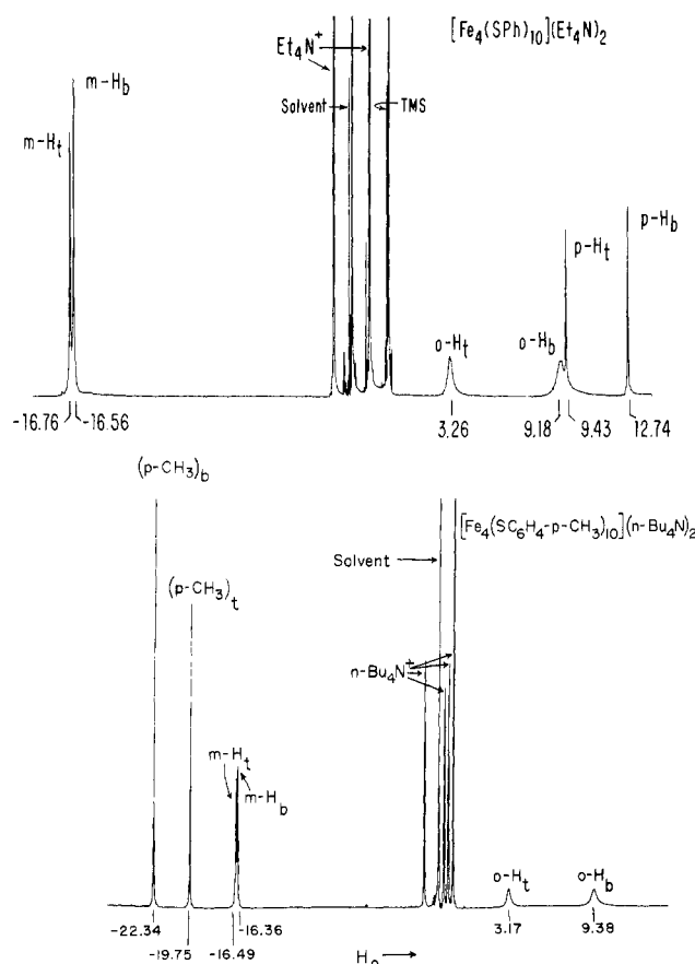
Figure 5. ^1\text{H} NMR spectra (360 MHz) in \text{CD}_3\text{CN} of (\text{Et}_4\text{N})_2[\text{Fe}_4(\text{SPh})_{10}] at -10^\circ\text{C} (top) and (n\text{-Bu}_4\text{N})_2[\text{Fe}_4(\text{S-}p\text{-tol})_{10}] at -5^\circ\text{C} (bottom). Signal assignments are indicated for bridging (b) and terminal (t) ligands.
