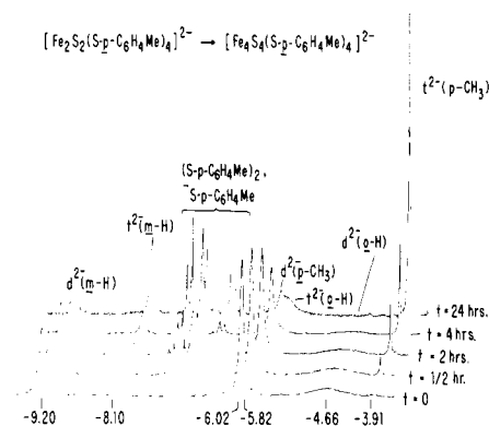
Figure 11. ^1\text{H} NMR spectra (100 MHz) demonstrating the conversion [\text{Fe}_2\text{S}_2(\text{S-p-tol})_4]^{2-} (\text{d}^{2-}) \rightarrow [\text{Fe}_4\text{S}_4(\text{S-p-tol})_4]^{2-} (\text{t}^{2-}) at \sim 27^\circ\text{C} . The reaction system at zero time consisted of 1 mL of 5 mM \text{d}^{2-} in \text{CD}_3\text{CN} + 0.5 mL of \text{CD}_3\text{OD} . Signal assignments are indicated.
