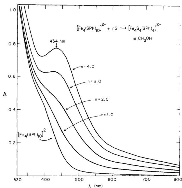
Figure 6. Visible spectra of equilibrium solutions resulting from the reactions of 5.00 mM \text{Na}_2[\text{Fe}_4(\text{SPh})_{10}] (from 20.0 mM \text{FeCl}_3 + 3.5 equiv of \text{NaSPh} ) with n = 1.0 –4.0 equiv of sulfur in \text{CH}_3\text{OH} at \sim 25^\circ\text{C} . Each spectrum corresponds to a separation reaction system measured 0.5–1 h after the addition of sulfur. The n = 4.0 curve corresponds to the spectrum of [\text{Fe}_4\text{S}_4(\text{SPh})_4]^{2-} .
