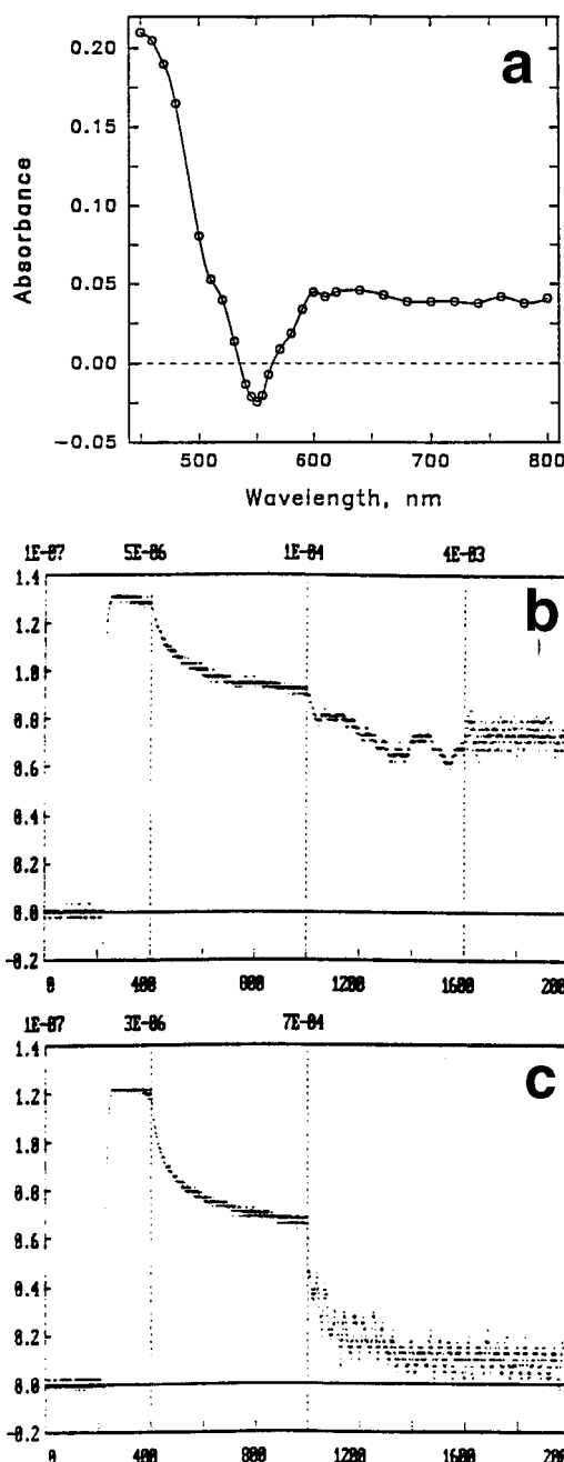
Figure 4. (a) Differential absorption spectrum recorded by pulse radiolysis of aqueous solutions containing 5 \times 10^{-5} \text{ mol L}^{-1} \text{ Fe}^{\text{II}}\text{TM2PyP} and 0.01 \text{ mol L}^{-1} \text{ HCOO}^- at pH 3.7, 20 \mu\text{s} after the pulse. (b) Absorbance ( \times 10 ) vs time over four time scales: 0.1 \mu\text{s} , 5 \mu\text{s} , 100 \mu\text{s} , and 4 ms per point, covering 2000 points, monitored at pH 8.6. (c) Absorbance ( \times 10 ) vs time over three time scales: 0.1, 3, and 700 \mu\text{s} per point, covering 2000 points, monitored in solutions containing bicarbonate and \text{CO}_2 at pH 6.7.
