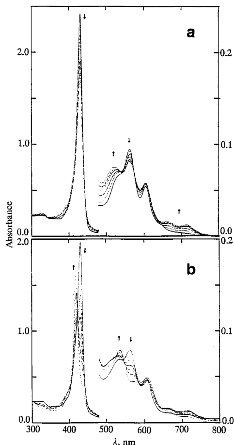
Figure 1. Photochemical reduction of \text{Fe}^{\text{III}}\text{TPP} ( 5 \times 10^{-5} \text{ mol L}^{-1} ) solutions in DMF containing 5% TEA: (a) under Ar and (b) under \text{CO}_2 . The arrows show bleaching of the \text{Fe}^{\text{III}}\text{TPP} absorptions and formation of the \text{Fe}^{\text{II}}\text{TPP} absorptions. Under \text{CO}_2 the absorptions of both \text{Fe}^{\text{II}}\text{TPP} and (\text{CO})\text{Fe}^{\text{II}}\text{TPP} are seen (see text).
