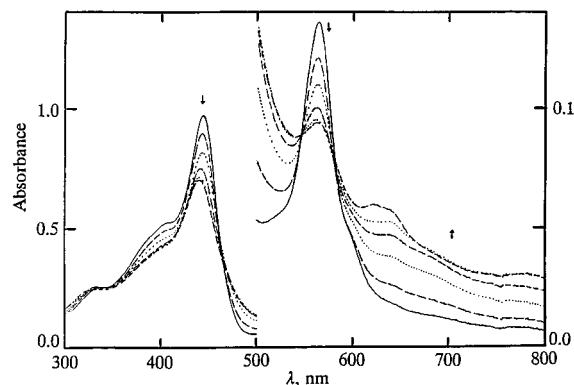
Figure 3. Radiolytic reduction of \text{Fe}^{\text{II}}\text{TM2PyP} ( 5 \times 10^{-5} \text{ mol L}^{-1} ) in deoxygenated aqueous solutions containing 0.1 \text{ mol L}^{-1} \text{ HCOO}^- and 1 \text{ mol L}^{-1} \text{ KOH} . The arrows show the stepwise increase or decrease in absorbance after each irradiation with a dose of 29 Gy.
