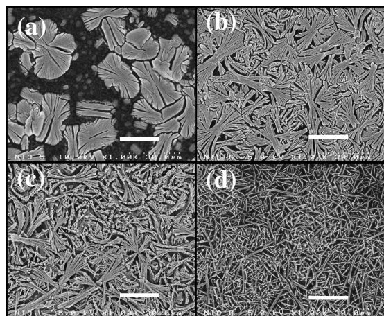
Figure 3. FE-SEM micrograph of porous NiO nanofiber on ITO. The amount of P123 is (a) 0.12 g, (b) 0.5 g, (c) 1.0 g, (d) 2.0 g. Scale bar and magnification is 24 \mu\text{m} and \times 1000 . Calcination temperature is 500 ^{\circ}\text{C} for 30 min.
