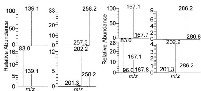
Figure 1. ESI-MS spectrum of irradiated solutions of 1 (after ethereal extraction) in neat 2a (top), in 2a containing 0.5 M pentenol (middle), and in 2e containing 0.5 M pentenol (bottom).
