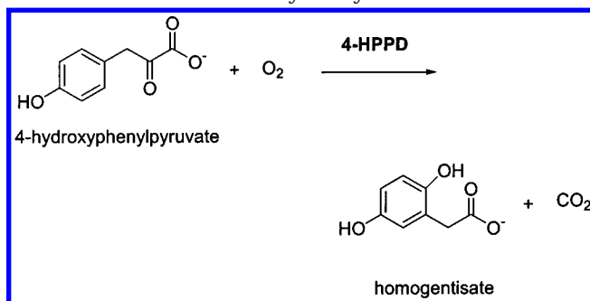
Scheme 1. Reaction Catalyzed by 4-HPPD
