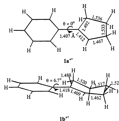
Figure 7. Optimized structure of monomer cation radicals of 1a,b obtained by semiempirical molecular orbital calculation with the PM3 method.
