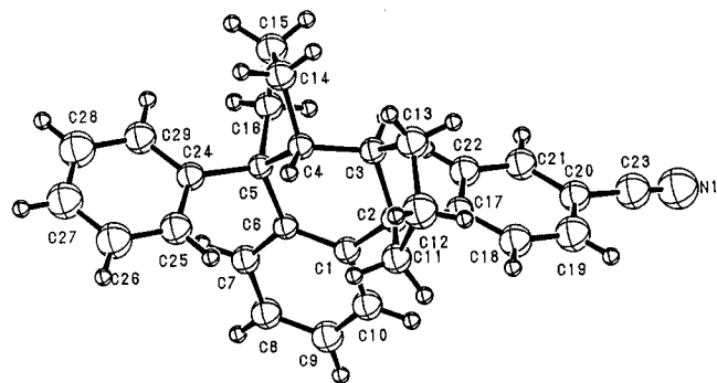
Figure 2. ORTEP drawing of adduct 5.
