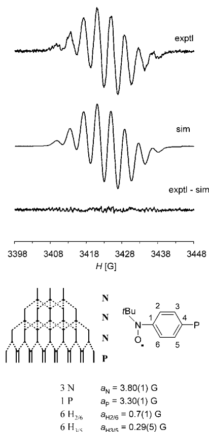
Figure 4. Top: Experimental and simulated EPR spectra of triradical 1 in fluid solution. Bottom: Stick diagram showing the eight overlapping lines along with the numbering scheme for 1 .
