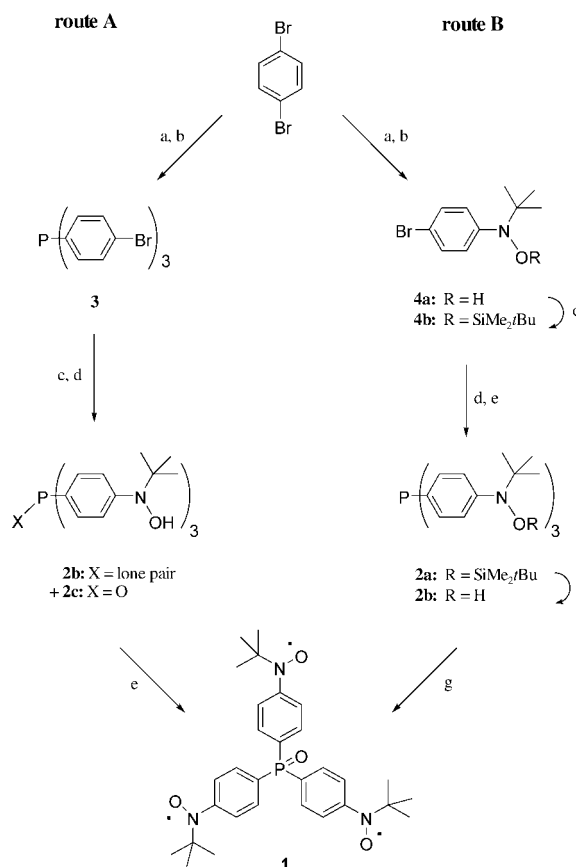
Scheme 1. Synthesis routes to triradical 1 . Route A: a) n BuLi; b) \text{PCl}_3 , c) n BuLi, d) (t\text{BuNO})_2 , e) \text{NaIO}_4 ; route B: a) n BuLi, b) (t\text{BuNO})_2 , c) \text{ClSiMe}_2t\text{Bu} , d) n BuLi, e) \text{PCl}_3 , f) \text{Bu}_4\text{NF} , g) \text{NaIO}_4 .
