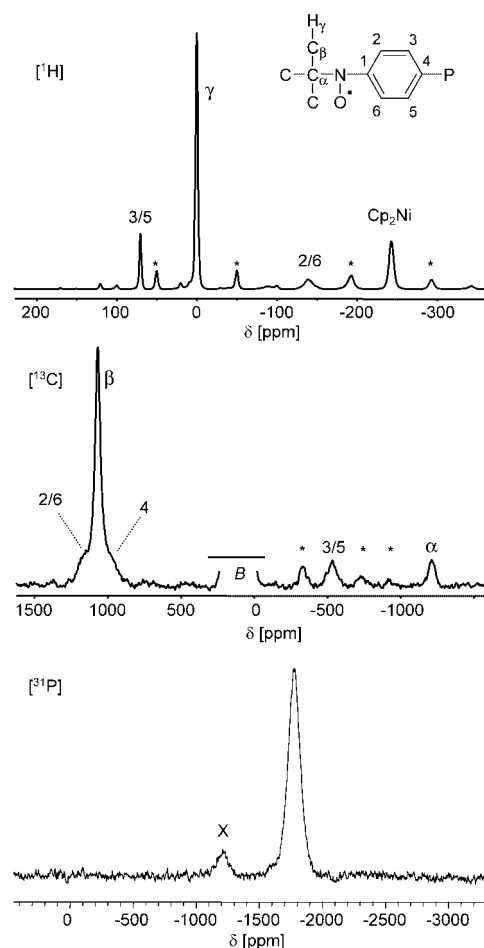
Figure 5. ^1\text{H} , ^{13}\text{C} , and ^{31}\text{P} MAS NMR spectra from top to bottom for triradical 1 ( T = 310.8 K, spinning rate: 15 kHz). Spinning side-bands are marked by asterisks. The signal of \text{Cp}_2\text{Ni} was used as internal temperature standard; X = impurity (probably the diradical derivative).
