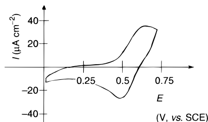
Figure 6. CV of a monolayer of 3e on an anodized Pt electrode, recorded in CH 3 CN/0.2 M TEAT.
