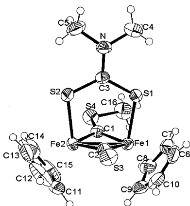
Fig. 2. Molecular structure of 3 showing the atomic numbering (thermal ellipsoids at 50% probability level).
