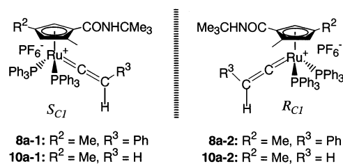
Fig. 3. A pair of enantiopore planar-chiral cyclopentadienylruthenium-vinylidene complexes 8 and 10 .
