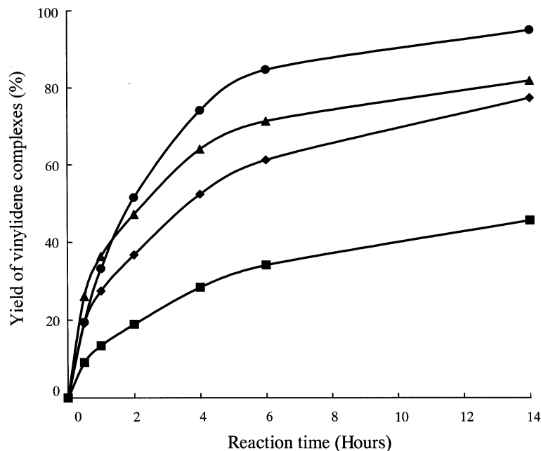
Fig. 4. Reaction rates of ruthenium complexes 11a with phenylacetylene derivatives \text{HCCC}_6\text{H}_4\text{R} . —▲—: \text{R} = \text{MeO} ; —◆—: \text{R} = \text{H} ; —■—: \text{R} = \text{NO}_2 ; —●—: The reaction of complex 14 with \text{HCCC}_6\text{H}_5 .
