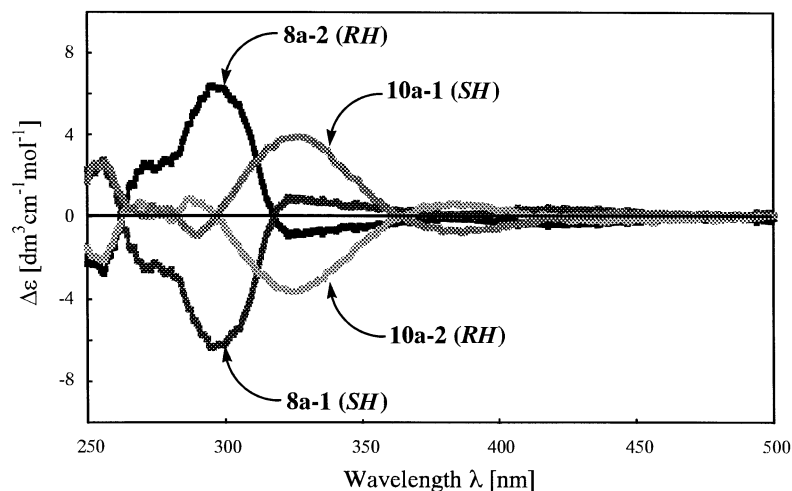
Fig. 2. CD spectra of ruthenium complexes 8a and 10a .
