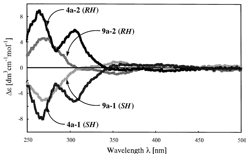
Fig. 1. CD spectra of ruthenium complexes 4a and 9a .
