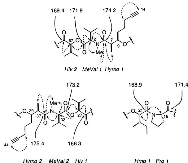
Figure 2. Selected HMBC correlations of onchidin B ( 4 ).
