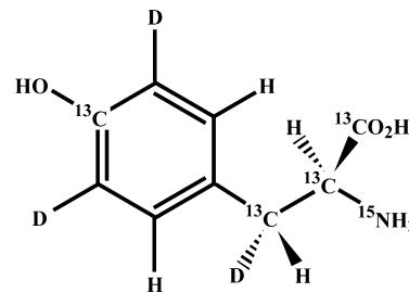
Figure 1. Stable isotope labeling pattern of SAIL (2S,3R)-[ \beta_2,\epsilon_{1,2} - ^2\text{H}_3 ;0, \alpha,\beta,\zeta - ^{13}\text{C}_4 ; ^{15}\text{N} ]-Tyr. ^{12}\text{C} atoms are not shown in the figure.
