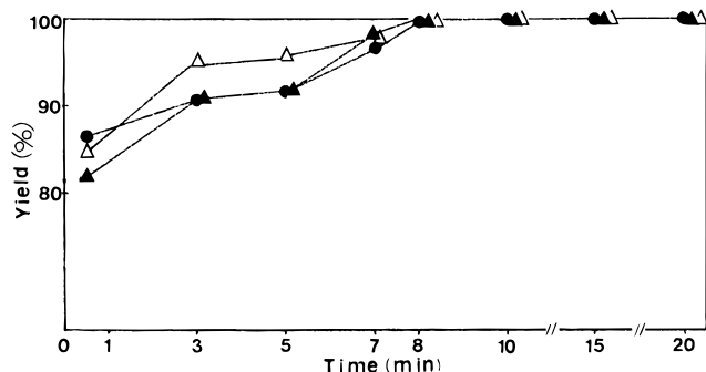
Figure 2. Effect of reaction time on derivatization of CAP (●), FF (▲), and TAP (Δ).
