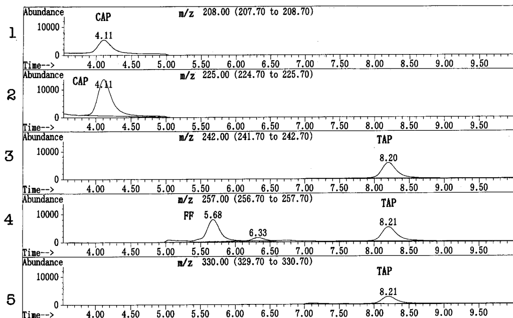
Figure 7. SIM of drug-fortified yellowtail muscle extract. Two micrograms of drug was added to 10 g of yellowtail muscle. Scan conditions were the same as described in Figure 6.
