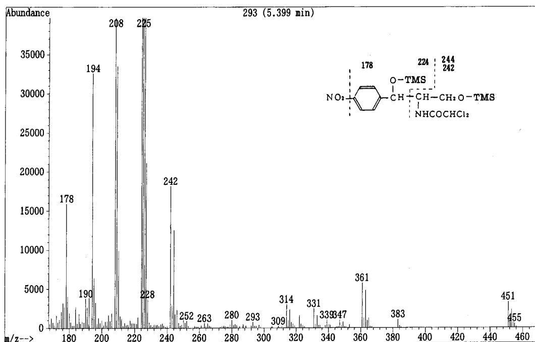
Figure 3. Mass spectrum of TMS derivative of CAP. Mass condition: ionization energy, 70 eV; electron multiplier, 1800 V; emission current, 300 \mu\text{A} ; scan range, 150–500.
