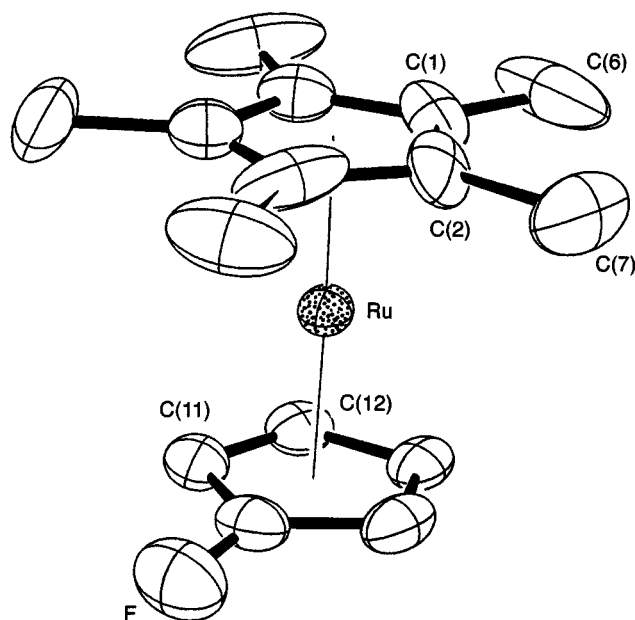
Figure 4. ORTEP diagram with labeling scheme for 17 . Thermal ellipsoids are drawn at 30% probability. The fluorine atom was located at three disordered positions with 56–28–16% distribution; only the 56% occupancy site is shown.
