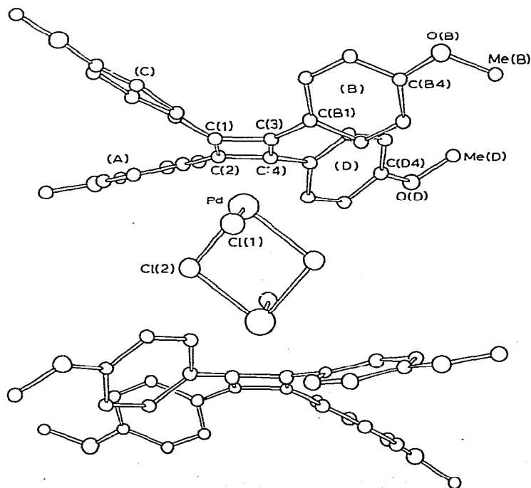
Fig. 1. The structure of [(\text{An}_4\text{C}_4\text{Pd})_2\text{Cl}_4] , complex 6 .
