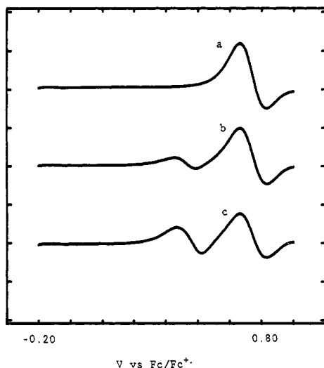
Figure 1. Linear sweep voltammograms for the oxidation of 4-chloro- N,N -dimethylaniline ( 1c ) (1.00 mM) in acetonitrile- \text{Bu}_4\text{NPF}_6 (0.1 M) at a voltage sweep rate of 0.1 V/s at 293 K. [\text{Bu}_4\text{NOAc}] = 0 (a), 0.25 mM (b), and 0.50 mM (c).
