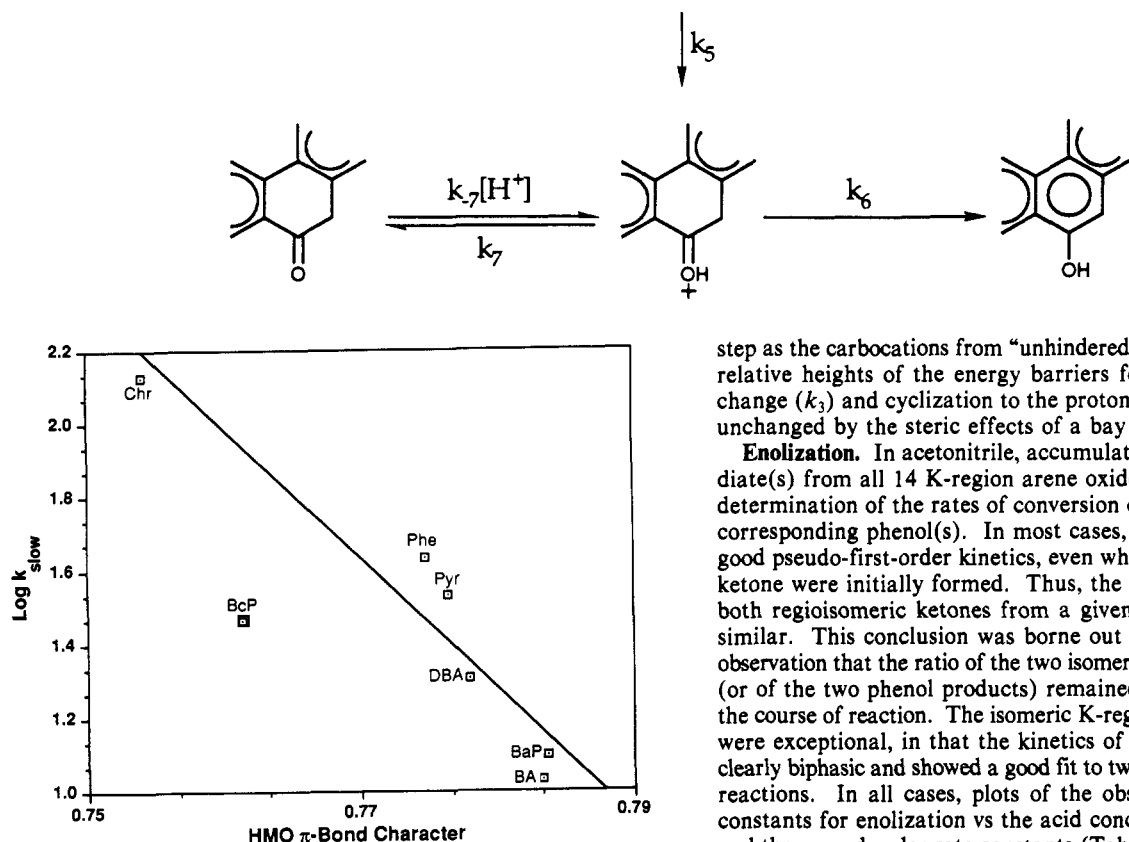
Figure 4. Plot of \log k_{\text{slow}} vs Hückel molecular orbital \pi -bond character calculated for the K-region bond of the parent hydrocarbon.
