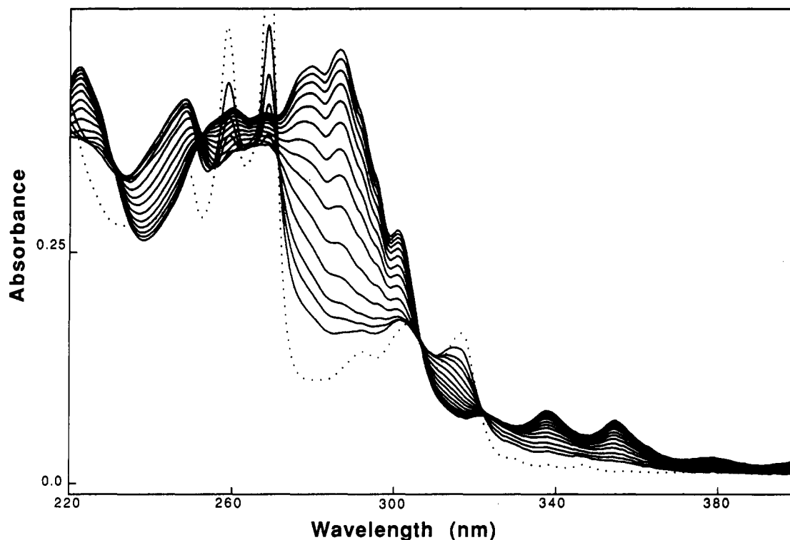
Figure 1. UV spectra measured as a function of time for the acid-catalyzed reaction of BA-O in acetonitrile ( 2.9 \times 10^{-4} M ethanesulfonic acid, at 25^\circ\text{C} ). The time interval is 10 s between the first five spectra and 60 s thereafter. The dotted line is the spectrum of the starting oxide.
